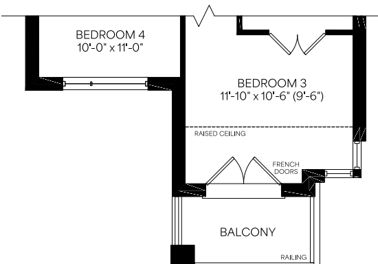
Second Floor Optional 4 Bedroom Plan Elevation C
