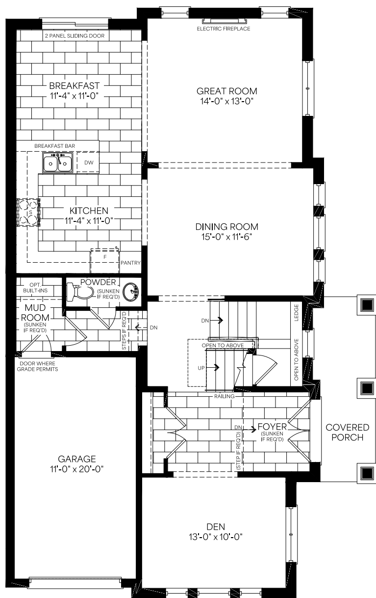
Main Floor Elevation A
