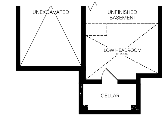
Basement Elevation B & C
