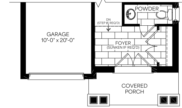
Main Floor Elevation B
