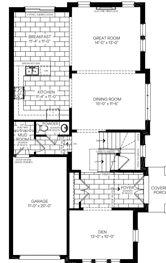
Main Floor Elevation B
