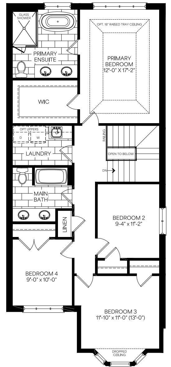
Second Floor Optional 4 Bedroom Plan Elevation A
