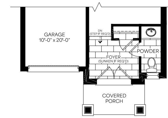
Main Floor Elevation B
